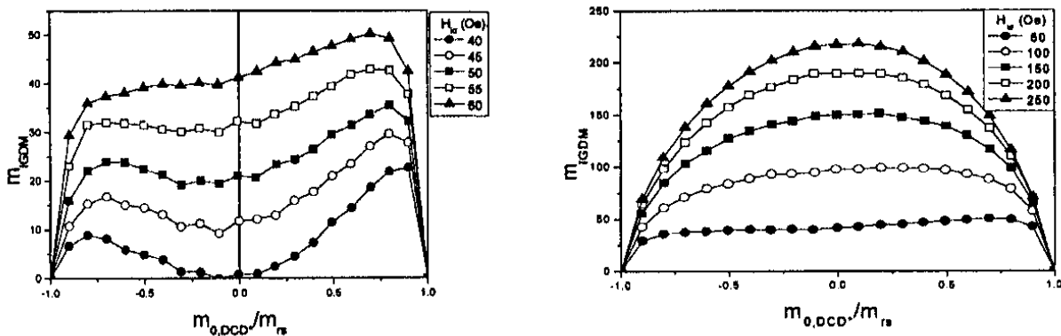
Fig. 3. Simulated IGDM with the GMP model with S = 0.85 ; \alpha = 90 Oe (the moving parameter); h_{c0} = 1160 Oe; h_{c\sigma} = 300 Oe; h_{r\sigma} = 2262 Oe; and for different values of the h_i parameter describing the interactions distribution (a) 40, 45, 50, 55 and 60 Oe., (b) 60, 100, 150, 200 and 250 Oe.
